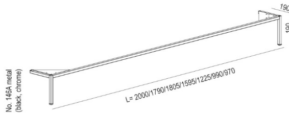
OPTION 2 1x FRAME No. 146a + 2 x LEG No.146
